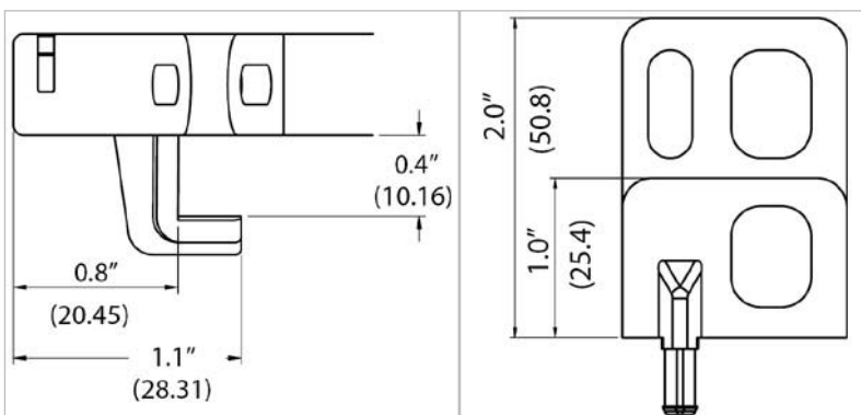
Hold-down tabs
